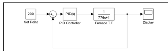
Figure 2 Simulink Model for PID Controller
