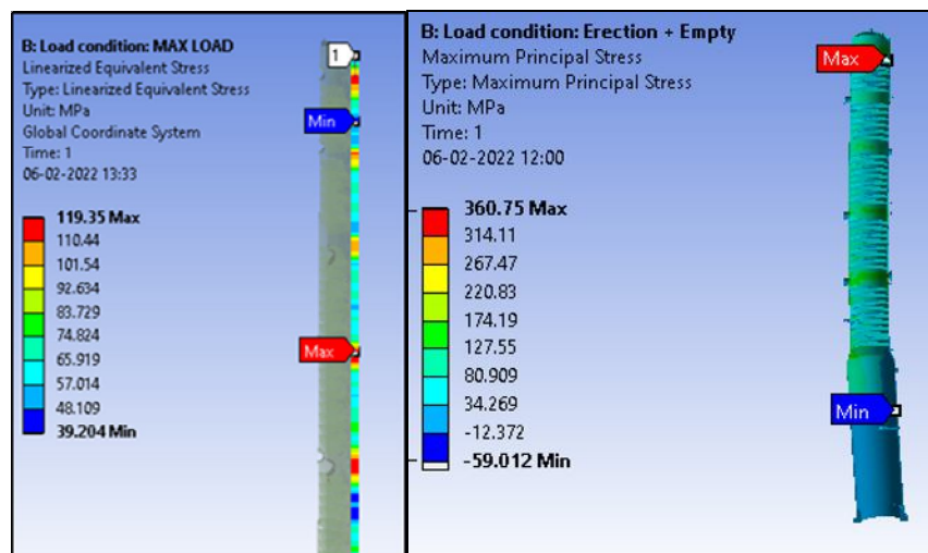
Figure 6. Contour plots foe equivalent stress & maximum principal stress for the tower
