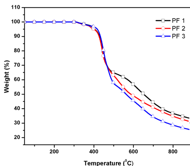
Fig. 3 Thermograms of polymers
