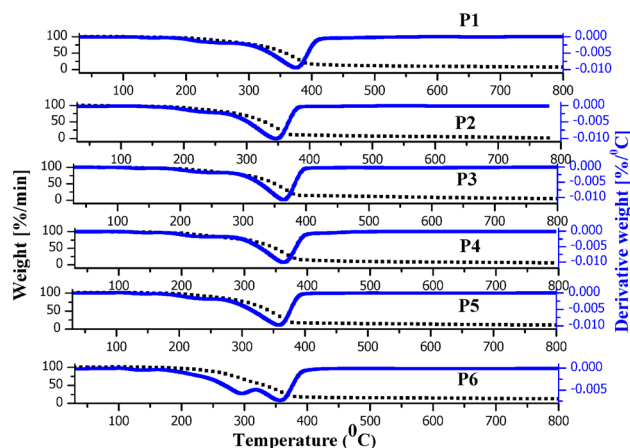
Fig. 5 Overlay thermograms of polymers
