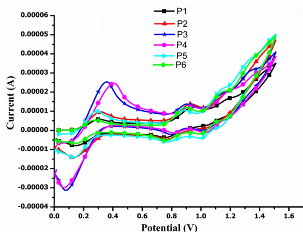
Fig. 6 Cyclic voltammograms of polymers ( P1–P6 ) in DCM using Ag/Ag + electrode calibrated with fc/fc + and TBAPF6 [tertiary butyl ammonium hexafluorophosphate (0.1 m)] as an electrolyte. The scan rate used was 50 mV S −1
